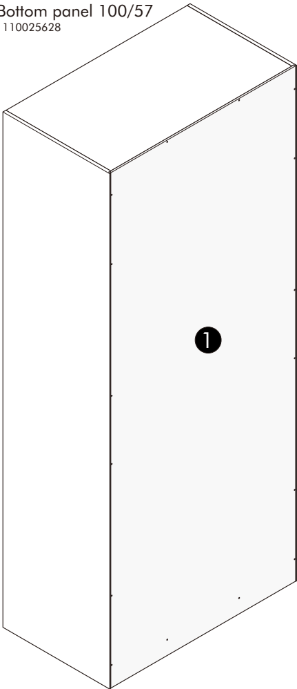
Side panel-L/R 57 110025623
